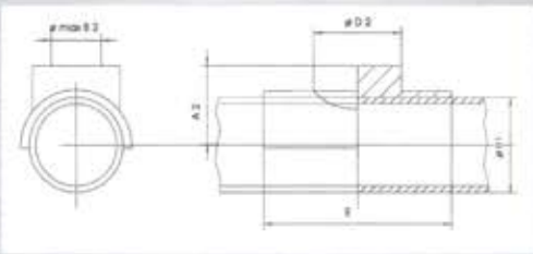
Saddle, Sattel, Demi-manchete de piquage
