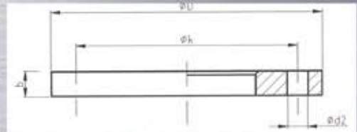
Loose Flange, Gf-Up-Losflansch, Bride Tournante
